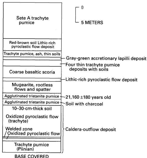
Figure 5. Measured stratigraphic section, roadcut on western wall of Sete Cidades caldera. All units dip approximately 17°W.
